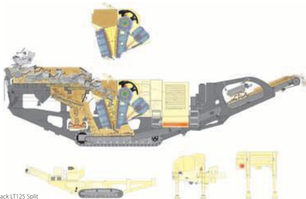
Lokotrack LT125 Split
